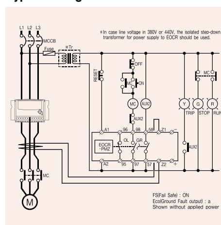
EOCR-PMZ (Terminal Type)
