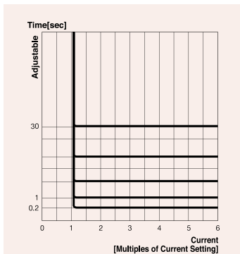
Definite Time Characteristic of EOCR-SP2/SS2/DS2(T)/DS3(T)
