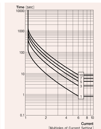
Inverse Time Characteristic of EOCR-SS1/DS1(T)
