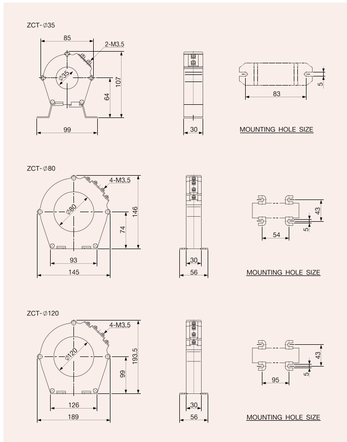
ZCT
